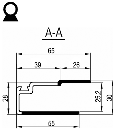
Edging profile for latch Hestal 681 S - TT 0423015.000
