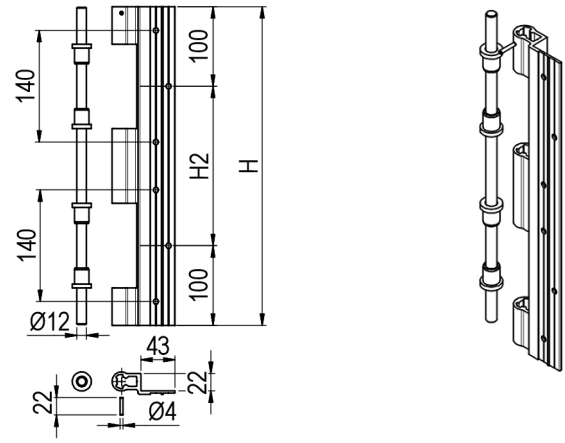
Riveting profile
